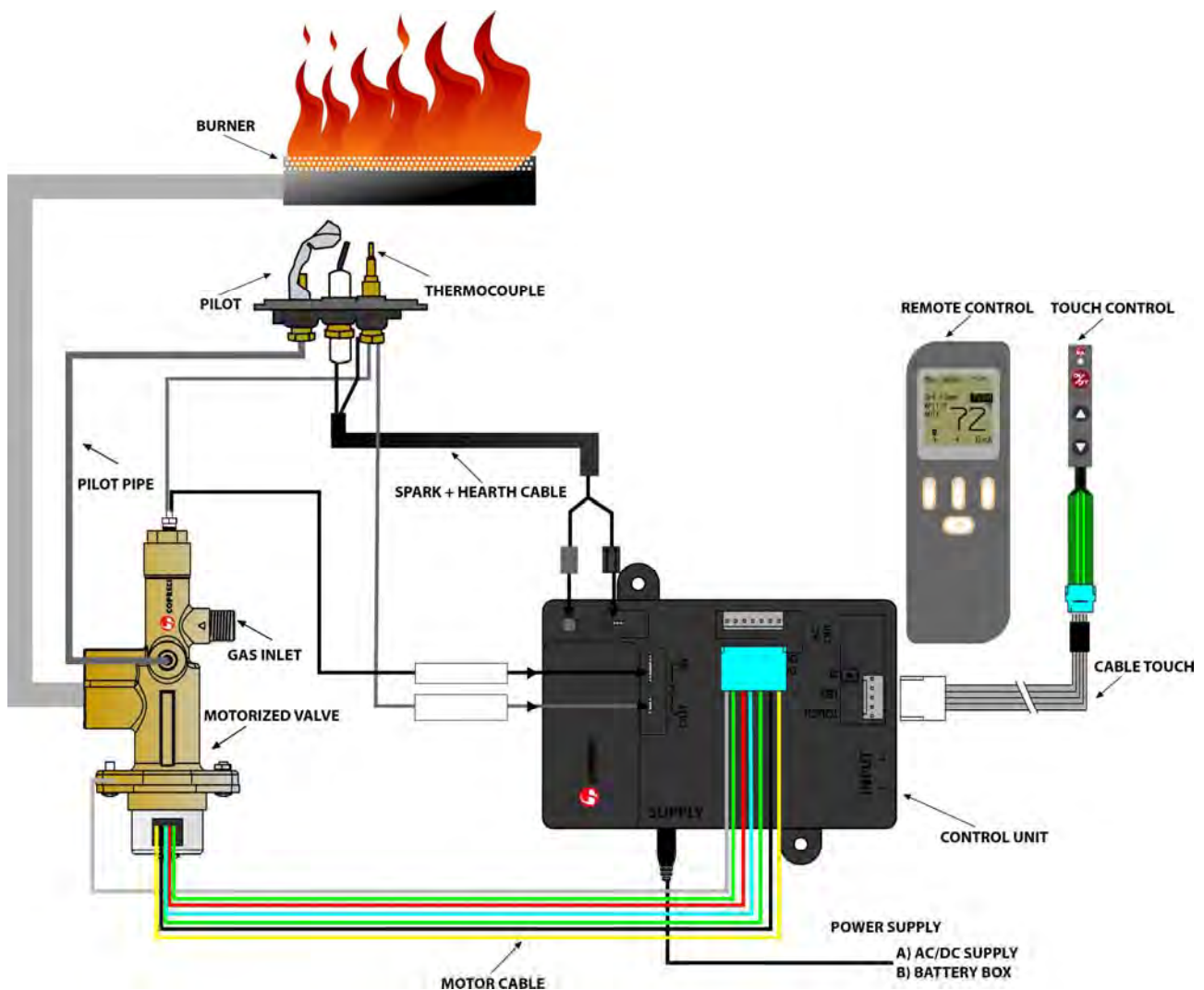
Figure 1. Connection scheme
