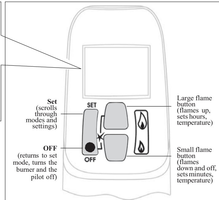
Handset Overview
